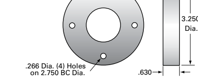
FLG7571 - Flanges FLG7571SS
