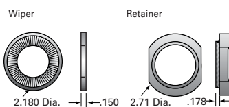
WKB2657 - 2 wipers/1 retainer
