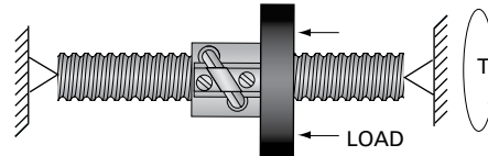
FIG. 12 - Holding Torque
