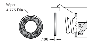
WKF3891 - 2 felt wipers/2 retainers
