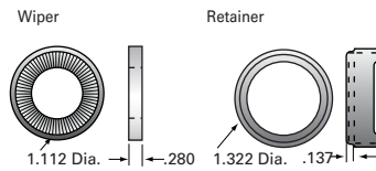
WKB2648 - 2 wipers/1 retainer
