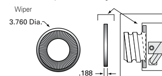
WKB2661 - 2 wipers/2 retainer rings
