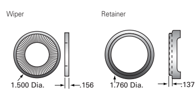
WKB2652 - 2 wipers/1 retainer
