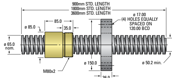
65 mm Trapezoidal Thread Lead Accuracy \pm 6.25 \mu\text{m}/25 \text{ mm}
