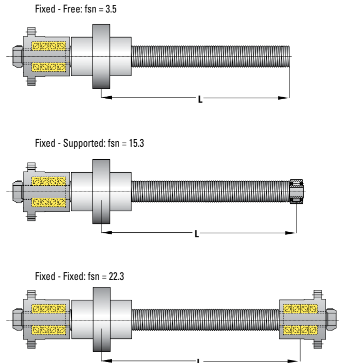
Fig. 3 - Critical Speed f_{sn} Factor
