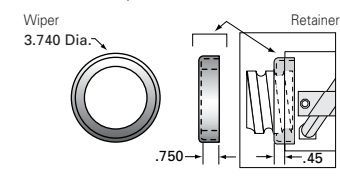
WKF3891 - 2 felt wipers/2 retainers
