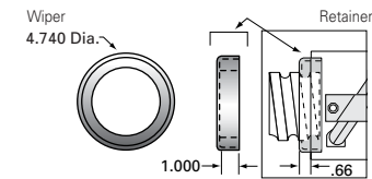
WKB3306 - 2 wipers/2 retainer rings
