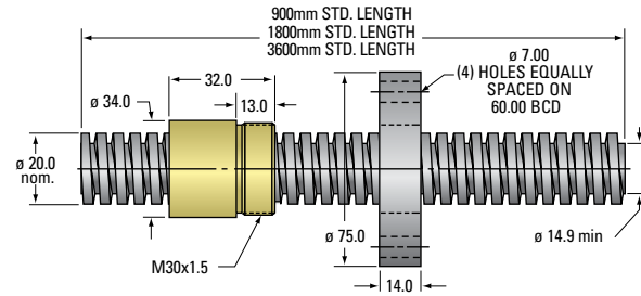
20 mm Trapezoidal Thread Lead Accuracy \pm 6.25 \mu\text{m}/25 \text{ mm}
