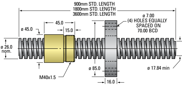
26 mm Trapezoidal Thread Lead Accuracy \pm 6.25 \mu\text{m}/25 \text{ mm}
