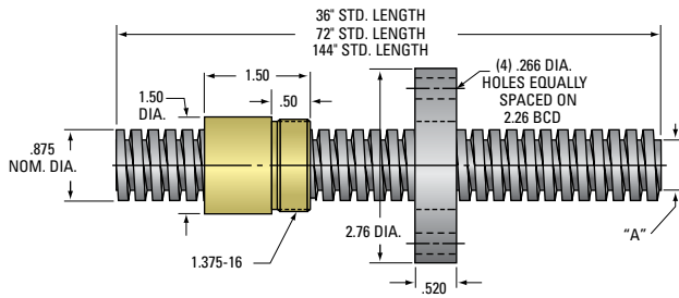
7/8" ACME THREAD Lead Accuracy 0.0003 in/in
