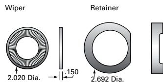
WKB2656 - 2 wipers/1 retainer
