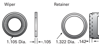
WKB7200 - 2 wipers/1 retainer
