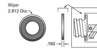
WKB2659 - 2 wipers/2 retainer rings
