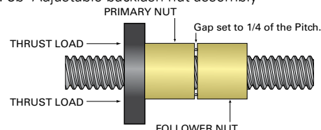
FIG. 3b Adjustable backlash nut assembly
