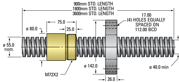
55 mm Trapezoidal Thread Lead Accuracy \pm 6.25 \mu\text{m}/25 \text{ mm}
